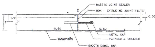
EXPANSION JOINT
