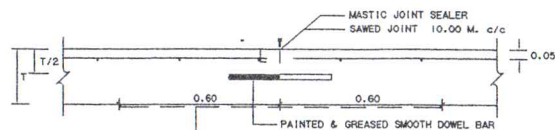
CONTRACTION JOINT
