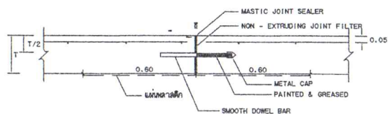
EXPANSION JOINT
